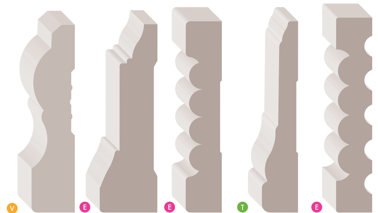
98063 3/4" x 3-1/4" PLDF 16' 00738 1" x 3-1/4" PLDF 16' 90908 5/8" x 3-5/16" PLDF 14', 16' 98233 5/8" x 3-5/16" PLDF 16' 90341 5/8" x 3-3/8" PLDF 14'
