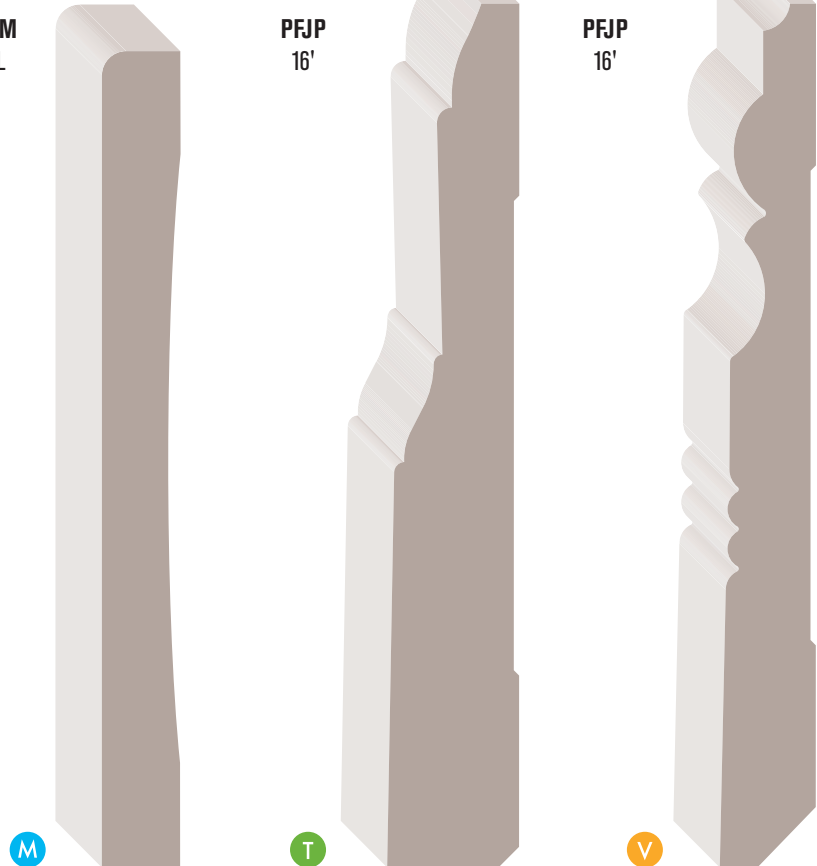
03707 7/16" x 4-1/4" HEM RL 00735 11/16" x 4-1/2" PFJP 16' 00964 1/2" x 4-1/2" PLDF 16'
