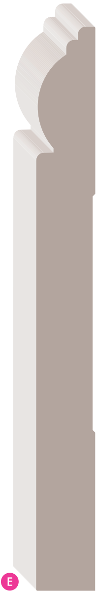
CR680 5/8" x 5-15/16" PLDF 16'
