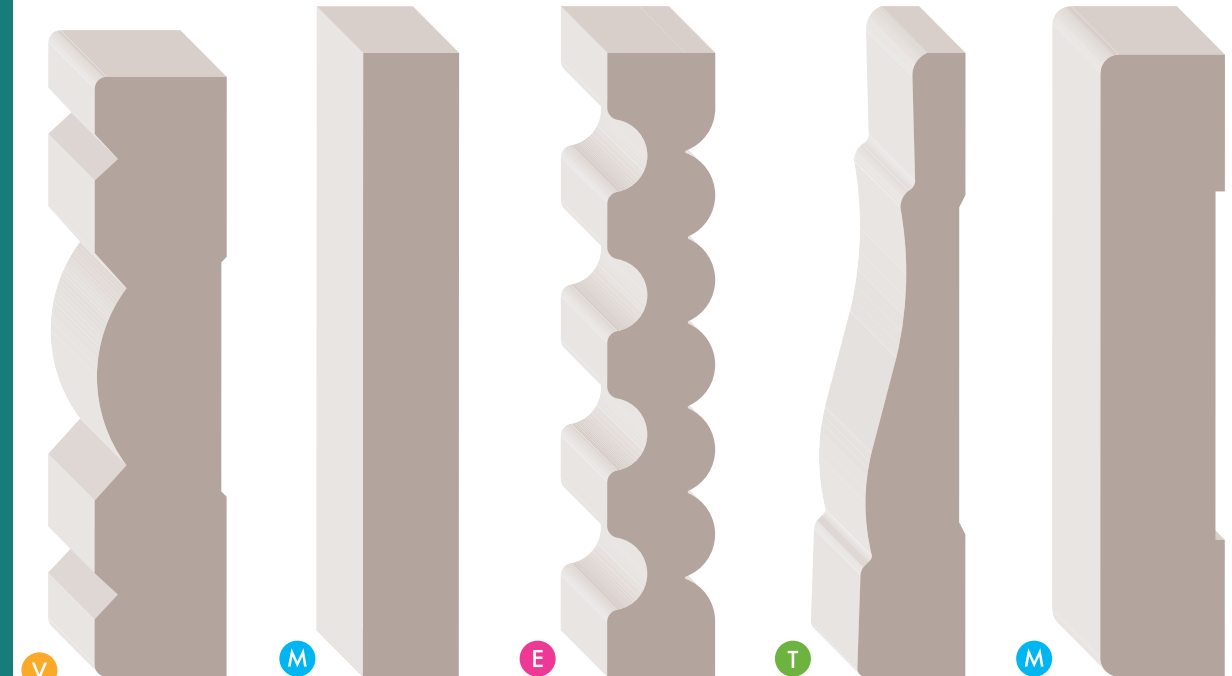
00729 11/16" x 3-1/8" PLDF 14', 16' W01X4 1/2" x 3-1/4" PLDF 16' 03125 9/16" x 3-1/4" PFJP 7'6", 15' HEM RL OH444 9/16" x 3-1/4" PLDF 16' HEM 8', RL 05126 5/8" x 3-1/4" KA RL PFJP 8', 16' KP 8', RL
