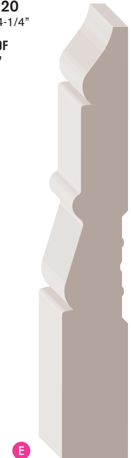
04312 11/16" x 4-1/2" PLDF 16'
