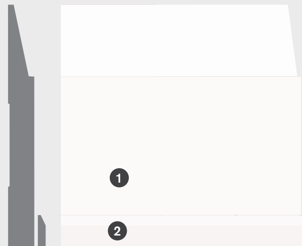
1 BAS-647 M BASEBOARD 11/16" x 6-1/4" AP
