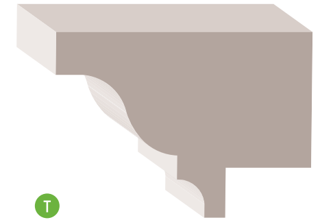
CAP-200 2-1/4" x 1-5/8" RABBET: 7/16" x 3/4" AP • WP • RO
