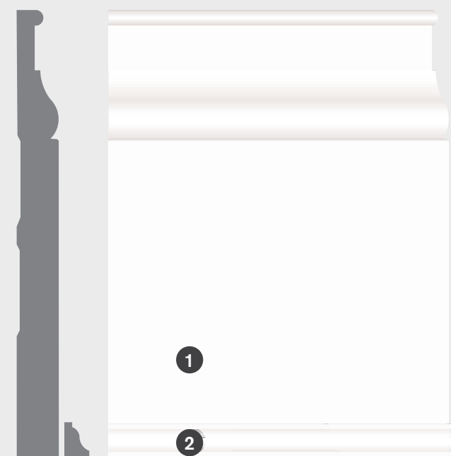
1 BAS-7A1 T BASEBOARD 11/16" x 7-1/4" AP
