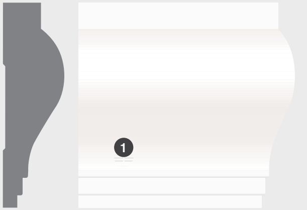
1 CAS-445 E CASING 1-5/16" x 4-1/4" AP
