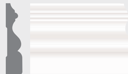
CAS-314 CASING 3/4" x 3-1/4" AP • PFJAP • WP RO • HM • KP
