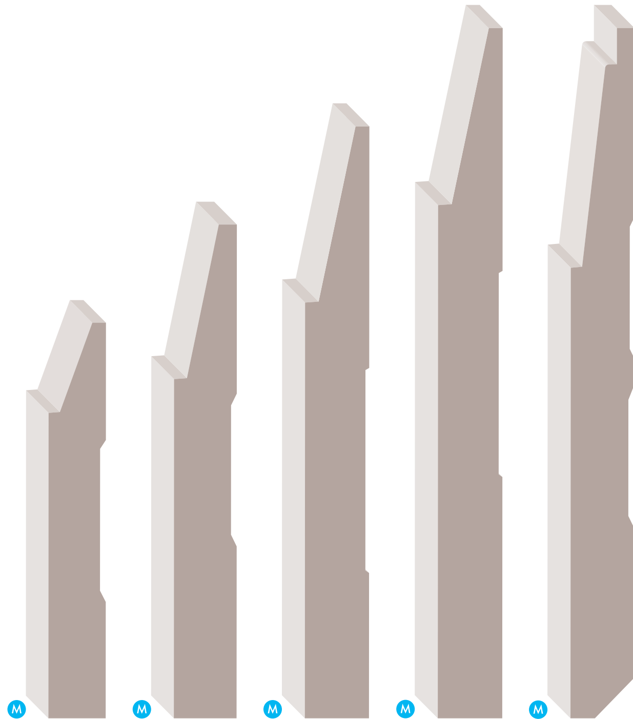
BAS-405 5/8" x 4-1/4" BAS-5M7 11/16" x 5-1/4" BAS-647 11/16" x 6-1/4" BAS-7A7 11/16" x 7-1/4" BAS-7K3 11/16" x 7-1/4" AP • PFJAP AP • PFJAP • FLEX 10' AP AP • PFJAP • WP FLEX 10' AP
