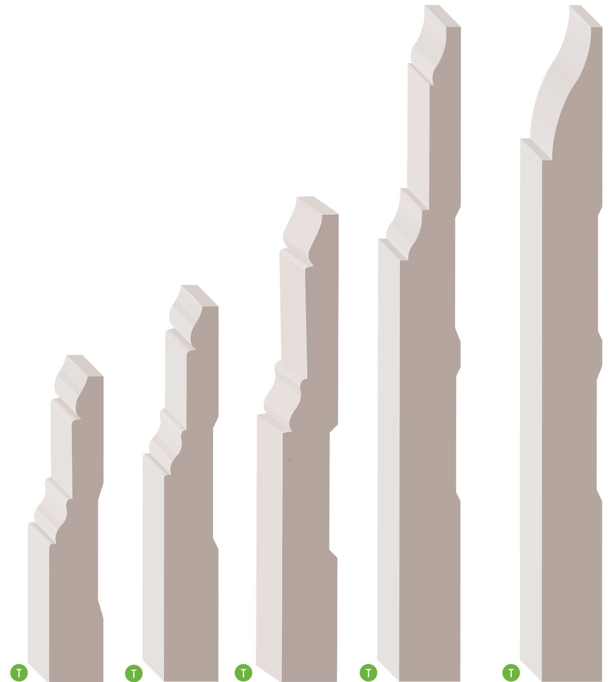
BAS-306 5/8" x 3-1/2" BAS-412 5/8" x 4-1/4" BAS-509 5/8" x 5-1/4" BAS-701 11/16" x 7-1/4" BAS-7K2 11/16" x 7-1/4" AP • RO • HM AP • PFJAP • WP RO • HM AP • PFJAP • WP RO • HM • FLEX 10' AP • PFJAP • WP RO • HM • FLEX 10' AP
