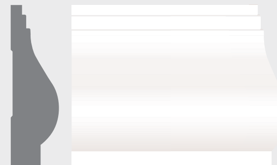
CAS-445 CASING 1-5/16" x 4-1/4" AP
