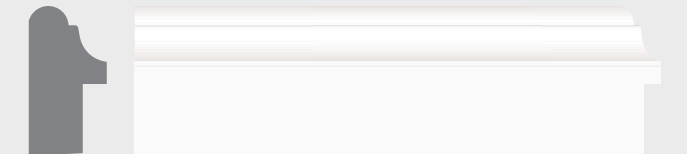
BAC-121 BACK BAND 13/16" x 1-9/16" AP • FLEX
